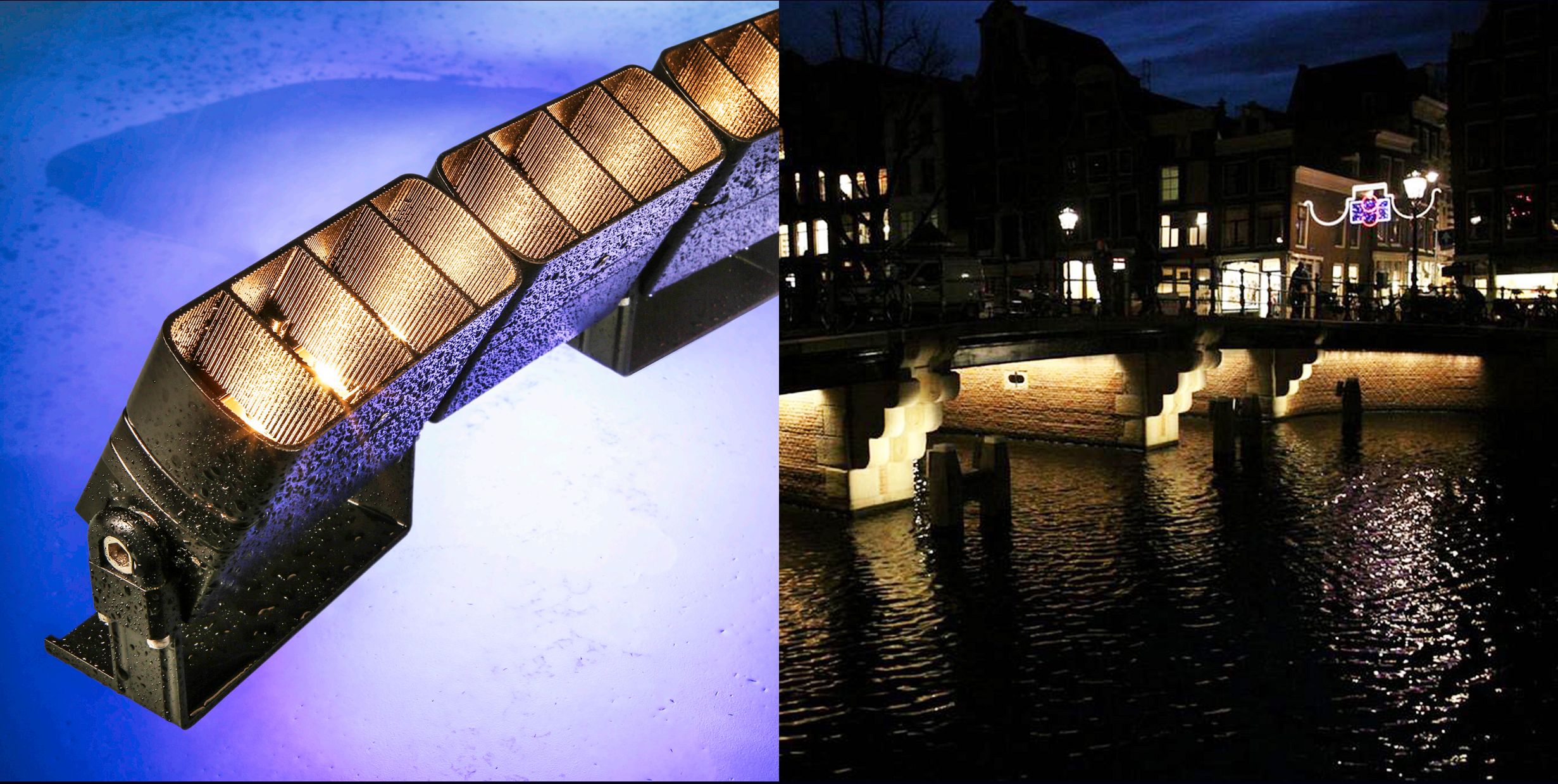
3D LED Flex 40 IP66 Modular, 3D flexible LED exterior linear lighting system Up to 5,000 Lumens per Mtr
